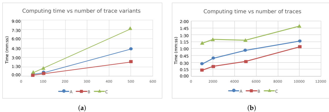
Figure 18. Performance of the greedy strategy when varying the log complexity. (a) Trace variants' complexity; (b) trace repetitions' complexity.
