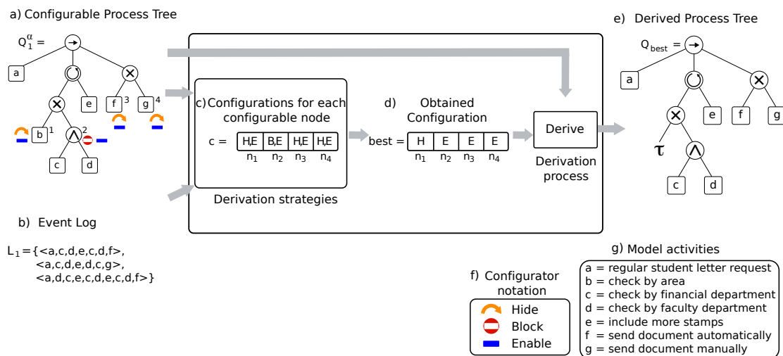
Figure 5. Running example that illustrates the derivation framework. A configurable process tree and an event log, shown in (a) and (b), are the inputs. The internal representation of a configuration used by the three strategies is represented in (c). The obtained configuration is shown in (d). Finally, the output, a derived process tree, is shown in (e).
