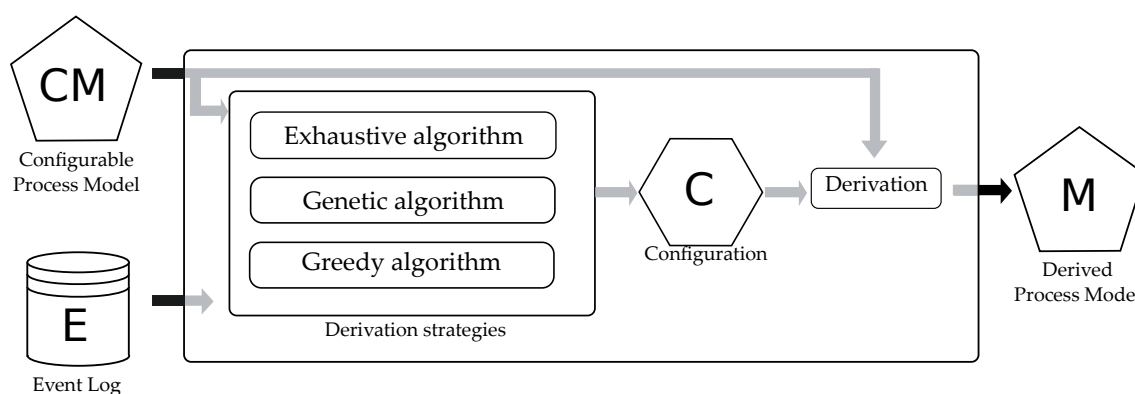
Figure 2. Overview of the proposed framework to derive a process model. Three alternative derivation strategies allow obtaining a configuration that later on is used to derive a process model from the configurable process model.
