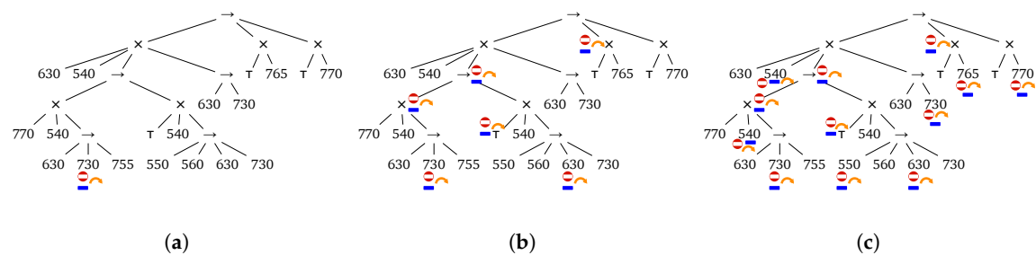
Figure 15. CPTs based on the model discovered by the ETM Approach 4. (a) CPT 4-A contains one configurable node; (b) CPT 4-B contains six configurable nodes; (c) CPT 4-C contains 12 configurable nodes.
