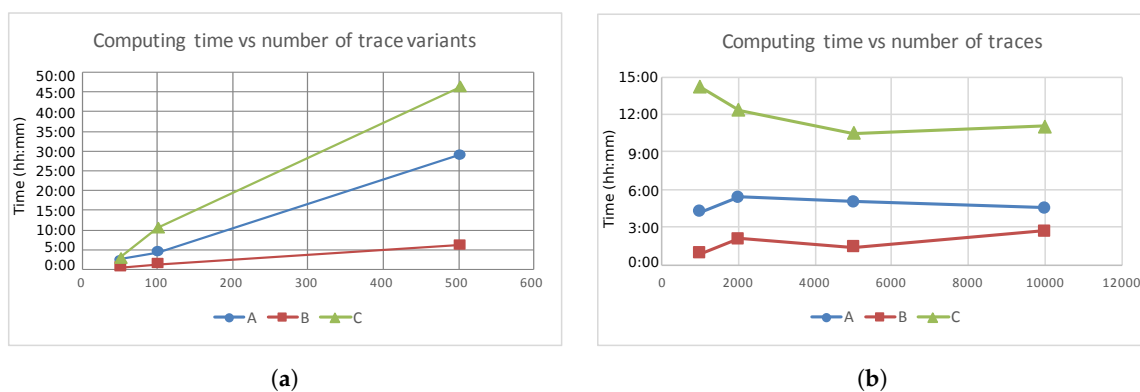
Figure 16. Performance of the exhaustive strategy when varying log complexity. (a) Trace variants' complexity; (b) trace repetitions' complexity.
