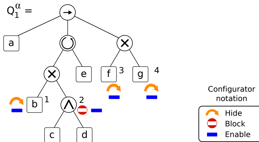
Figure 4. Example of a configurable process tree containing four configurable nodes.
