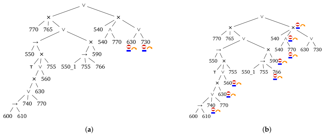
Figure 14. CPTs based on the model discovered by the ETM Approach 3. (a) CPT 3-A contains two configurable nodes; (b) CPT 3-B contains eight configurable nodes.
