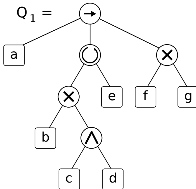
Figure 3. Example of a process tree model.
