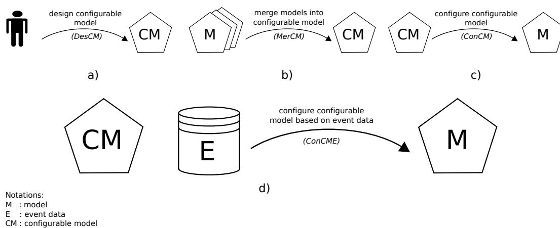
Figure 1. Business process management (BPM) use cases [7] related to configurable process models: (a) manually design a configurable process model (DesCM), (b) merge the collection of process models to generate a configurable process model (MerCM) and (c) configure a configurable process model (ConCM) to obtain a process model. In this article, we propose (d) as a new use case: to derive a process model based on a configurable process model and using event data (ConCME).
