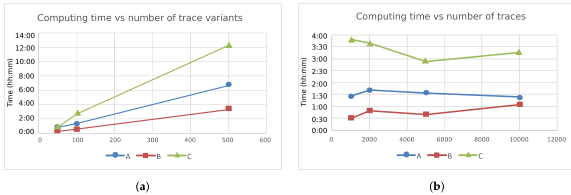
Figure 17. Performance of the genetic strategy when varying log complexity. (a) Trace variants complexity; (b) trace repetitions' complexity.
