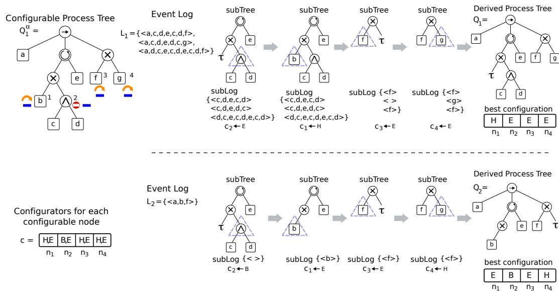
Figure 9. Overview of the greedy strategy to derive a process tree. There are two event log inputs to show different subtree and sub-log scenarios to finally derive a process tree.
