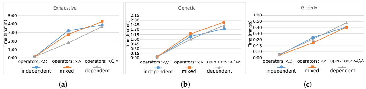
Figure 19. Performance of the different strategies when varying the model complexity. (a) Exhaustive; (b) genetic; (c) greedy.
