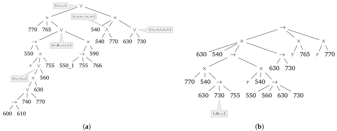
Figure 13. Process trees originally discovered by the evolutionary tree miner (ETM) on the building permits process event logs. (a) ETM Approach 3; (b) ETM Approach 4.
